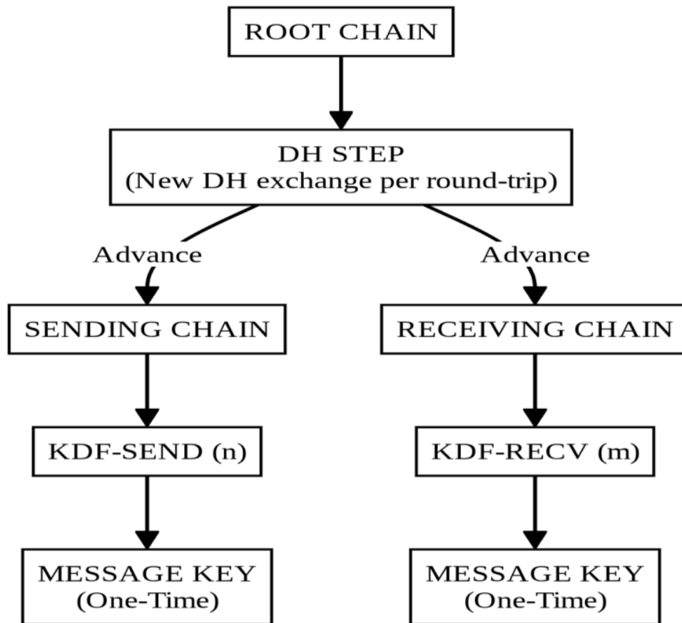
Figure 3: The Double Ratchet Protocol
