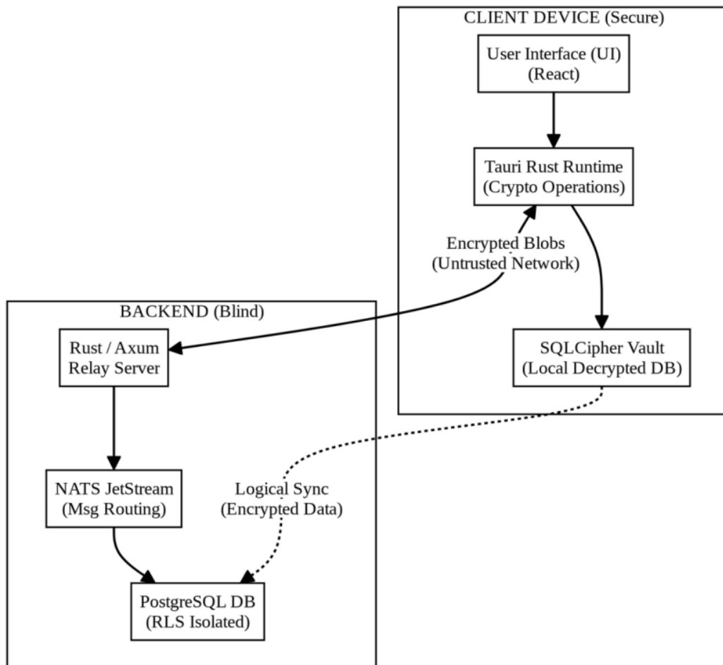
Figure 1: Zero-Knowledge "Blind Router" Logic
