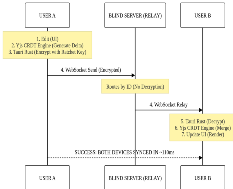
Figure 6: CRDT Synchronization Flow
