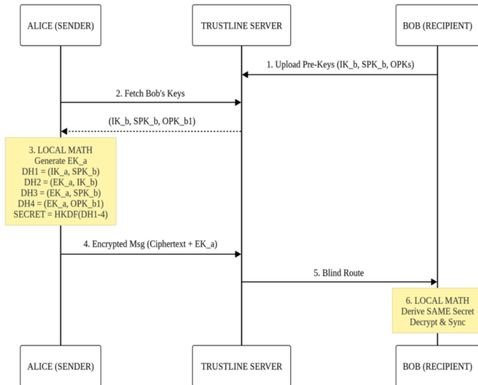
Figure 2: X3DH Key Agreement
